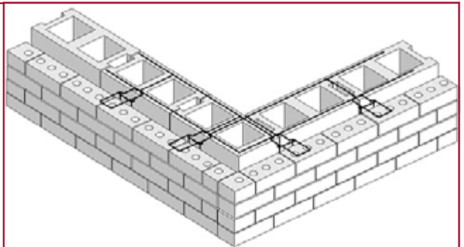
PREFABRICATED CORNER
