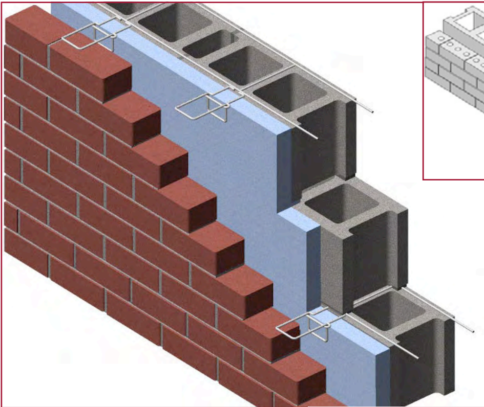
16" O.C. cross rods allow core clearance.
